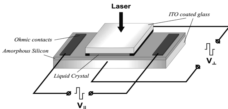
Figure 4. The view of investigated NLC cell.
